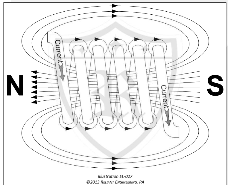
Basic Inductor Coil
